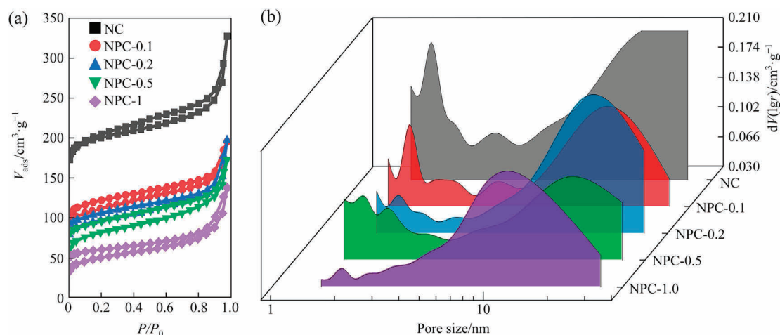
Fig. 5. (a) \text{N}_2 sorption isotherms and (b) pore size distribution of NC and NPC-x samples.
