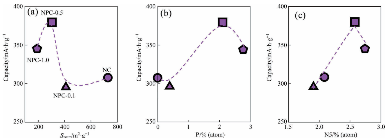
Fig. 7. Electrochemical performance as a function of the specific surface area (a), the surface concentrations of P content (b) and N5 species (c).
