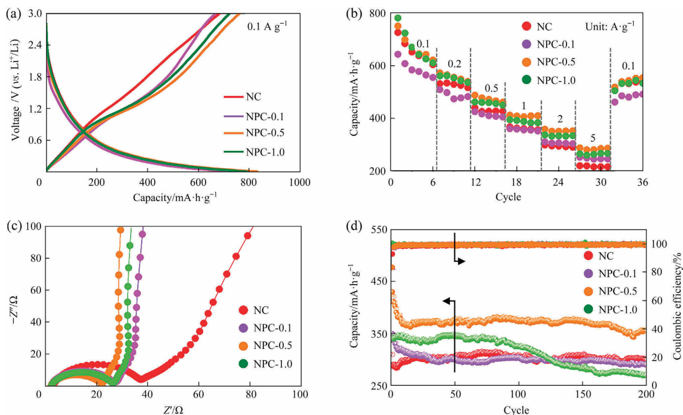
Fig. 6. Electrochemical performance of NC and NPC-x as anodes for lithium ion batteries in \text{LiPF}_6 electrolyte in the potential of 0.01 to 3.0 V versus \text{Li}^+/\text{Li} . (a) GCD profiles measured at 0.1 \text{ A} \cdot \text{g}^{-1} . (b) Rate capability recorded at different current densities from 0.1 to 5 \text{ A} \cdot \text{g}^{-1} . (c) EIS plots. (d) Cycling performance tested at 2 \text{ A} \cdot \text{g}^{-1} . For the convenience of comparison, the initial Coulombic efficiency was reported in Fig. S5.
