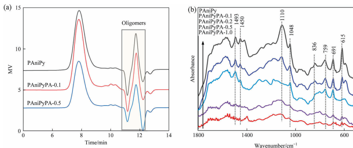
Fig. 2. (a) GPC profiles and (b) FTIR spectra of PAniPy and PAniPyPA- x samples.
