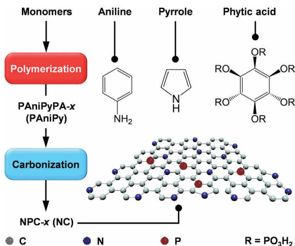
Fig. 1. Synthetic strategy of the polyaniline-based polymers via oxidative polymerization of ternary monomers and the corresponding nanocarbon materials accompanied with the sample codes.
